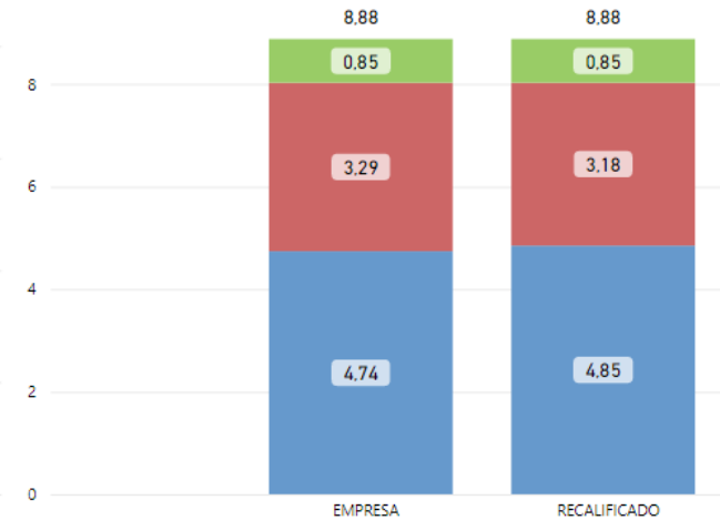
SAIDI 2021
