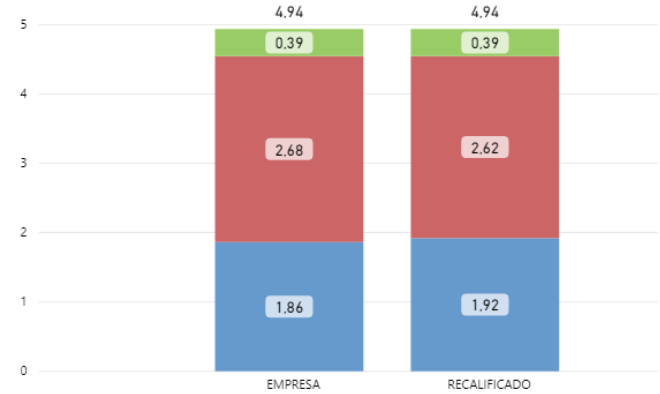
SAIDI 2021
