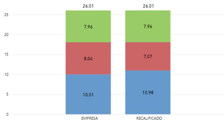
SAIDI 2021
