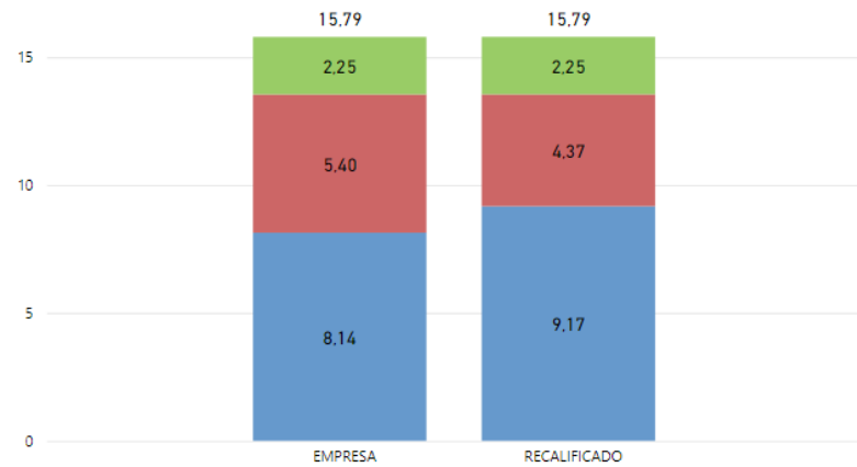
SAIDI 2021
