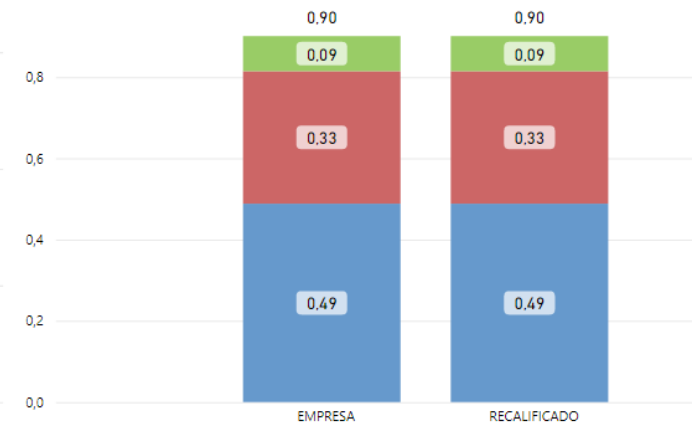
SAIDI 2022
