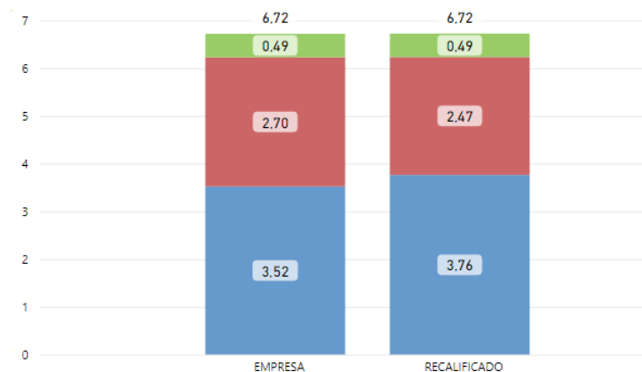
SAIDI 2022
