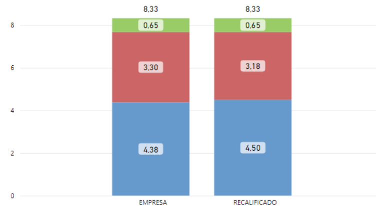
SAIDI 2023
