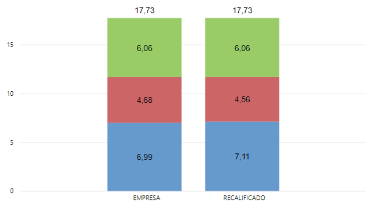
SAIDI 2022
