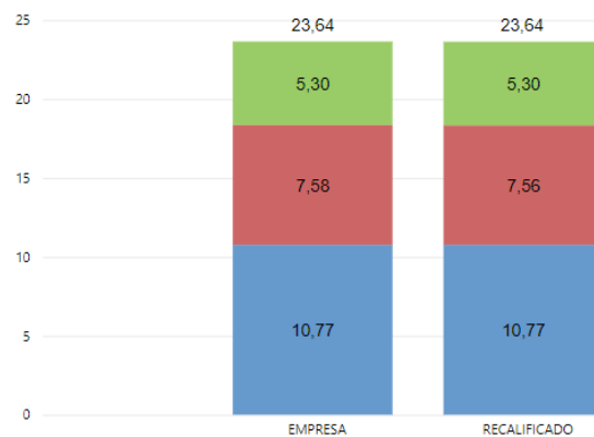
SAIDI 2024
