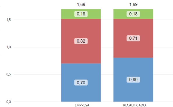
SAIDI 2024
