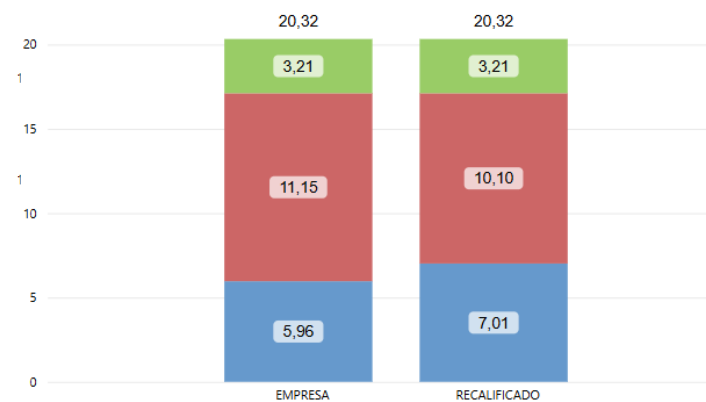
SAIDI 2024
